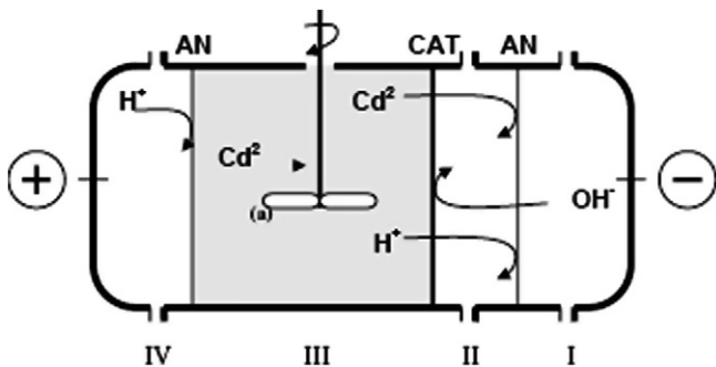
Figure 13 Electrodesion remediation of cadmium from wastewater sludge (Jakobsen et al., 2004) (AN: anion exchange membrane, CAT: cation-exchange membrane, (a) stirrer).
