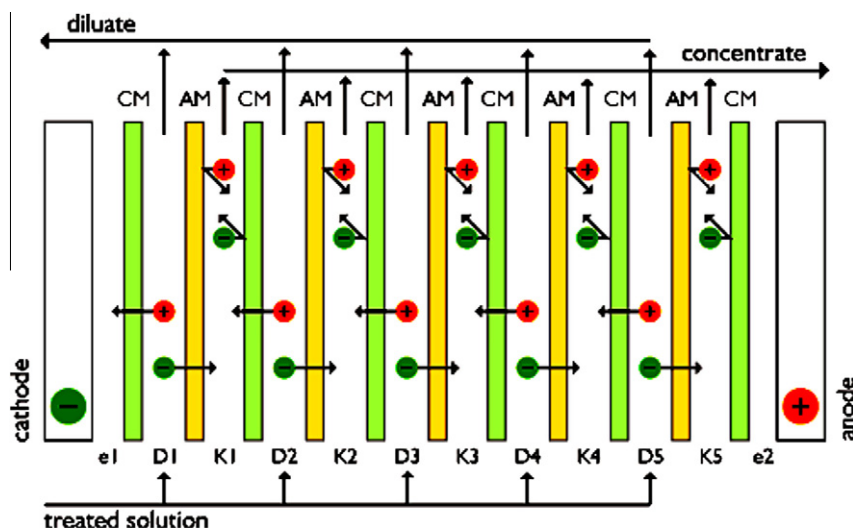
Figure 12 Electrodesion principles (Chen, 2004). CM – cation-exchange membrane, D – diluate chamber, e1 and e2 – electrode chambers, AM – anion exchange membrane, and K – concentrate chamber.
