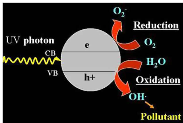
Figure 14 The conceptual reaction path of photocatalysis over TiO 2 (Herrmann, 1999).
